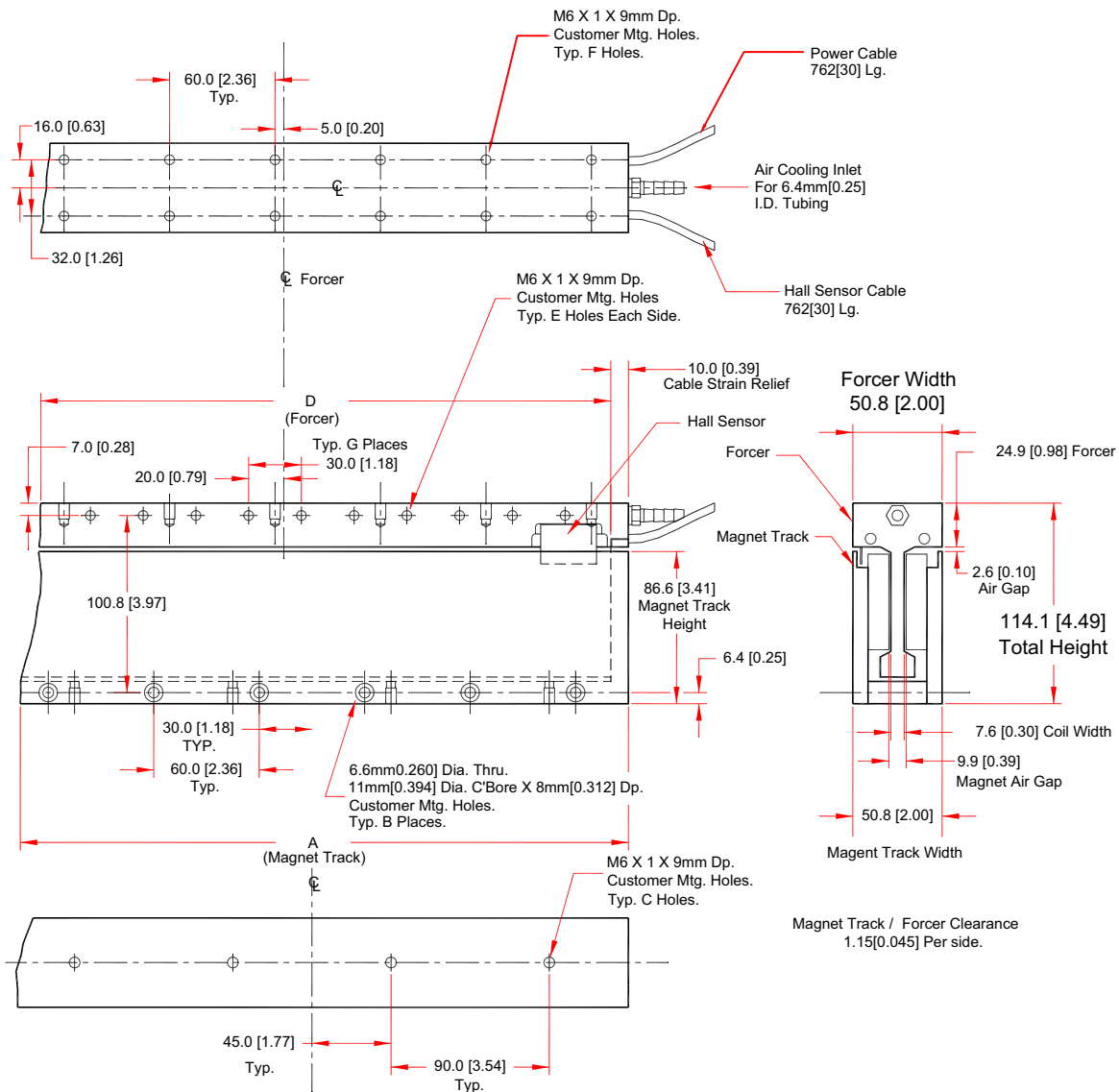
Dimensions - millimeters [inches]
